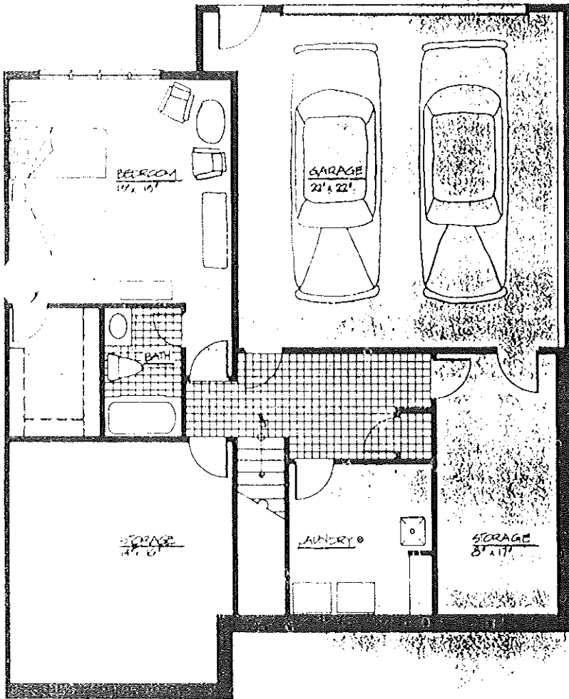
BASEMENT / GARAGE
