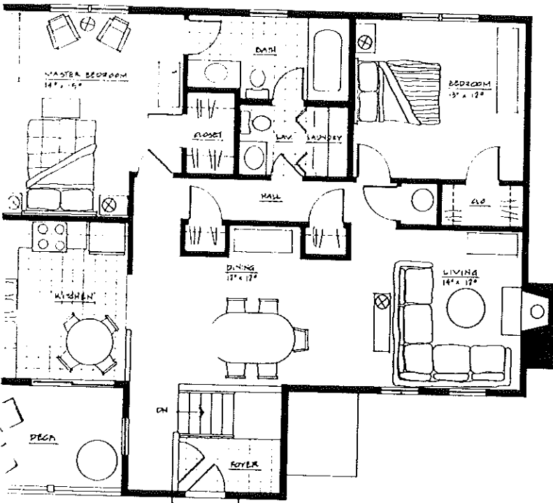
UPPER LEVEL PLAN
